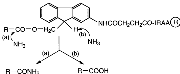
Scheme 4. Base- or nucleophile-promoted cleavage of the peptide-resin bond yields the target product as the C-terminal acid or C-terminal carboxamide, respectively.
